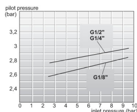
Actuation pneumatic/spring
