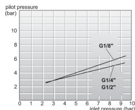
Actuation pneumatic/internal pilot air
