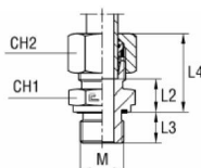
with B4 cutting ring
