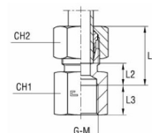
with B3 cutting ring
