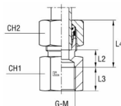
with B4 cutting ring
