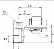
with B4 cutting ring
