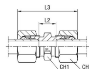
with B3 cutting ring
