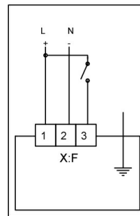
2-point control
