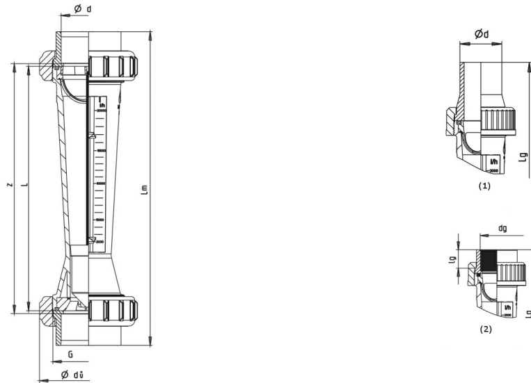
(1)...Fitting with welding nipple, (2)...Fitting with threaded sleeve
