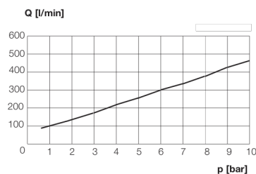
Flow rate
