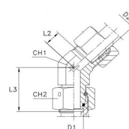
with B3 cutting ring
