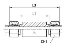
with B3 cutting ring
