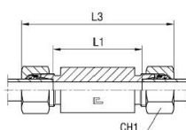
with B4 cutting ring
