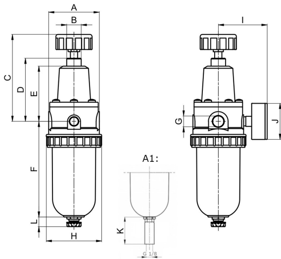
A1: automatic drain valve
