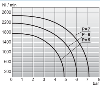
Flowdiagram 1/4"
